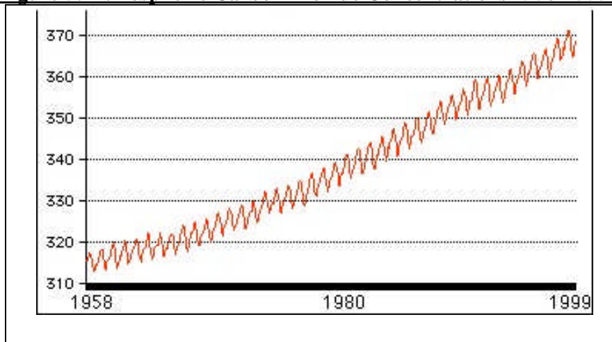
Figure 5: Atmospheric Carbon Dioxide Concentrations 1958–1999 46
